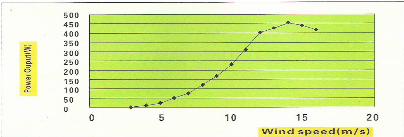
HYWG-400 Wind Speed -Output Power Curvy
