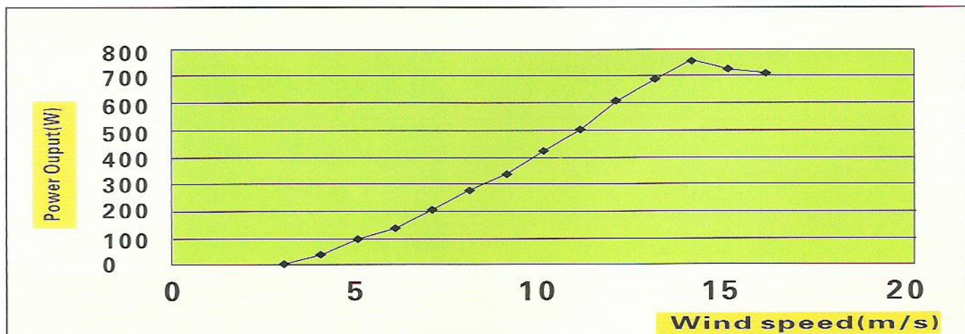
HYWG-600 Wind Speed-Output Power Curve
